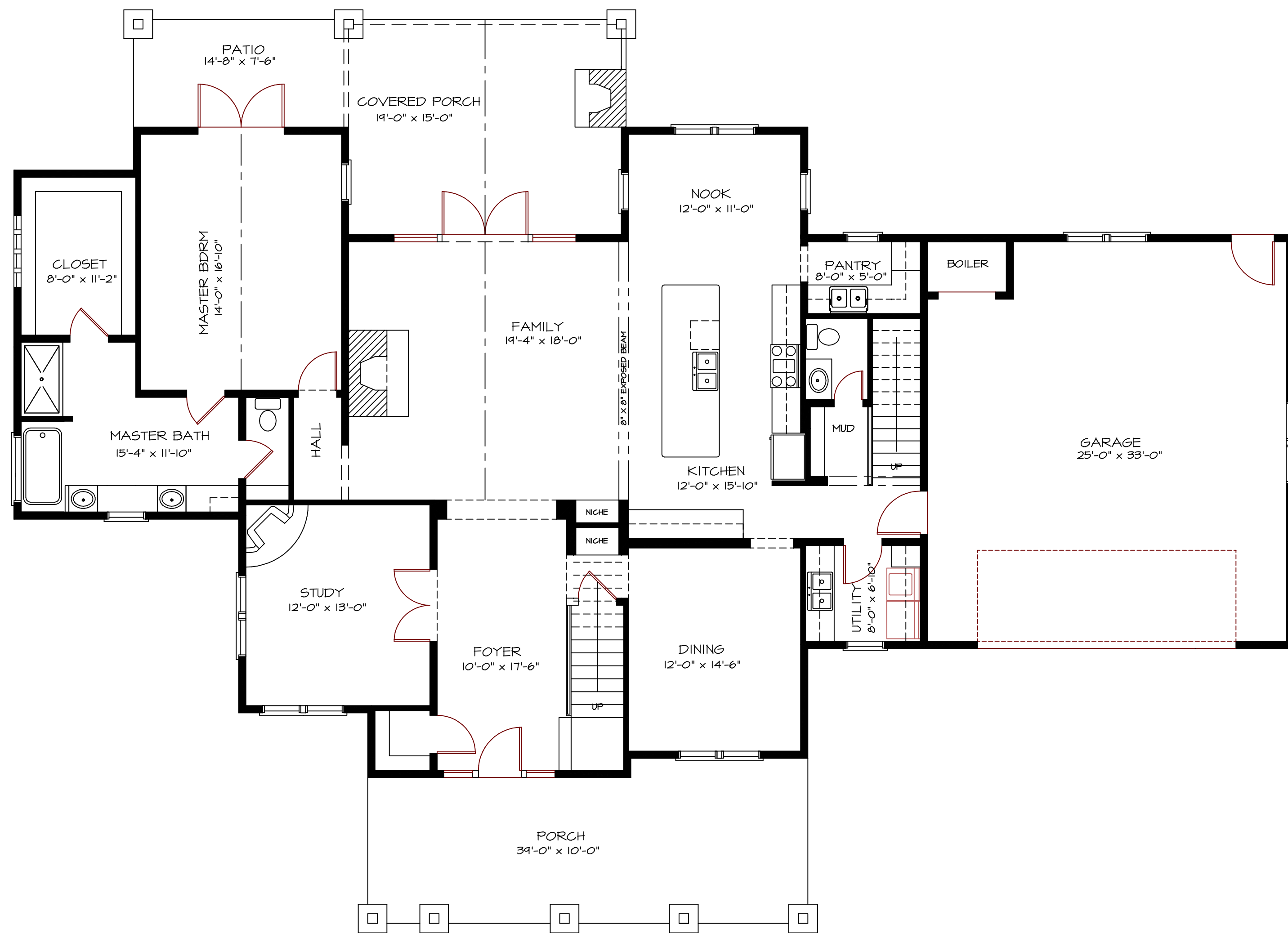
MAIN FLOOR PLAN NOT TO SCALE
