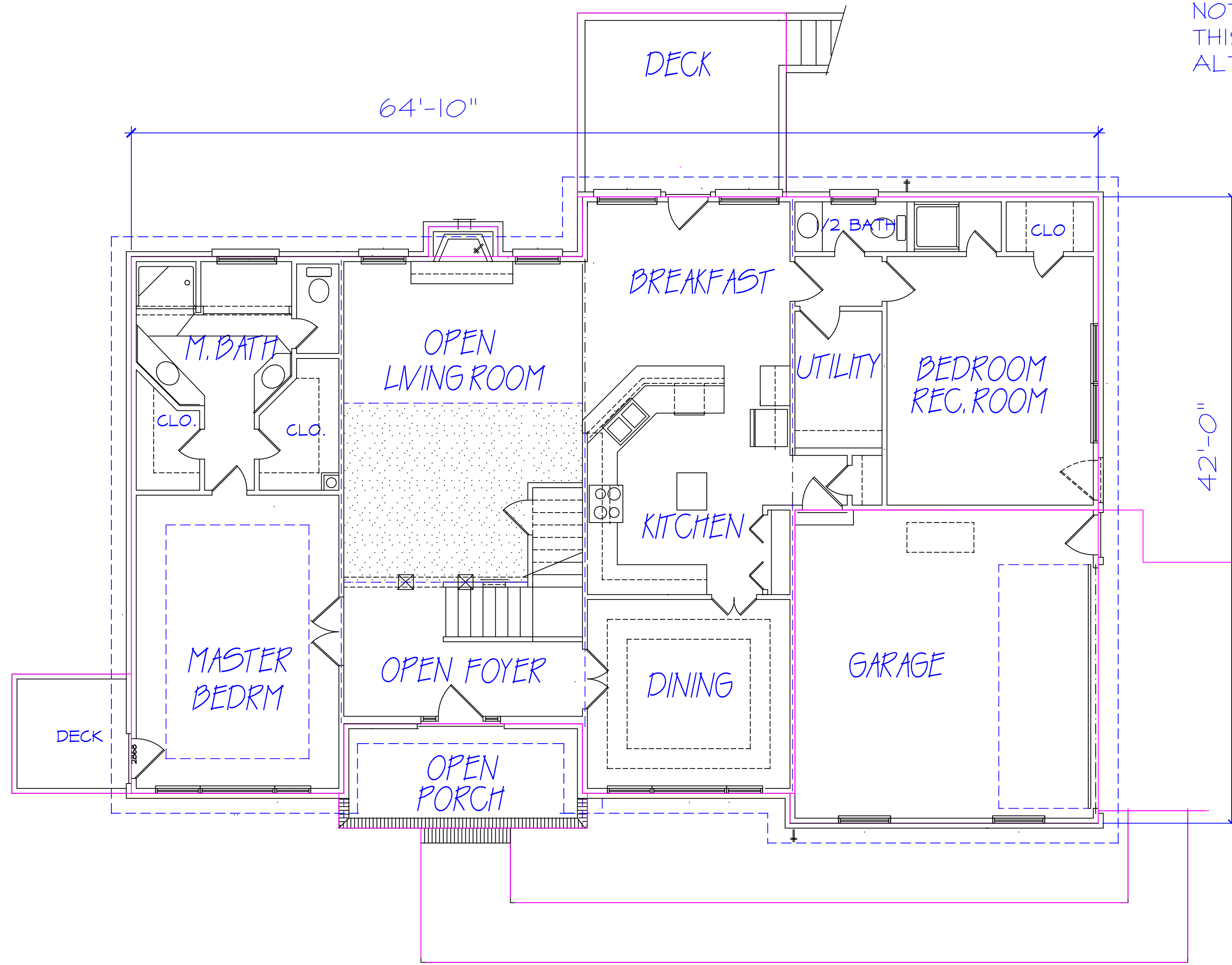
MAIN FLOOR PLAN NOT TO SCALE
