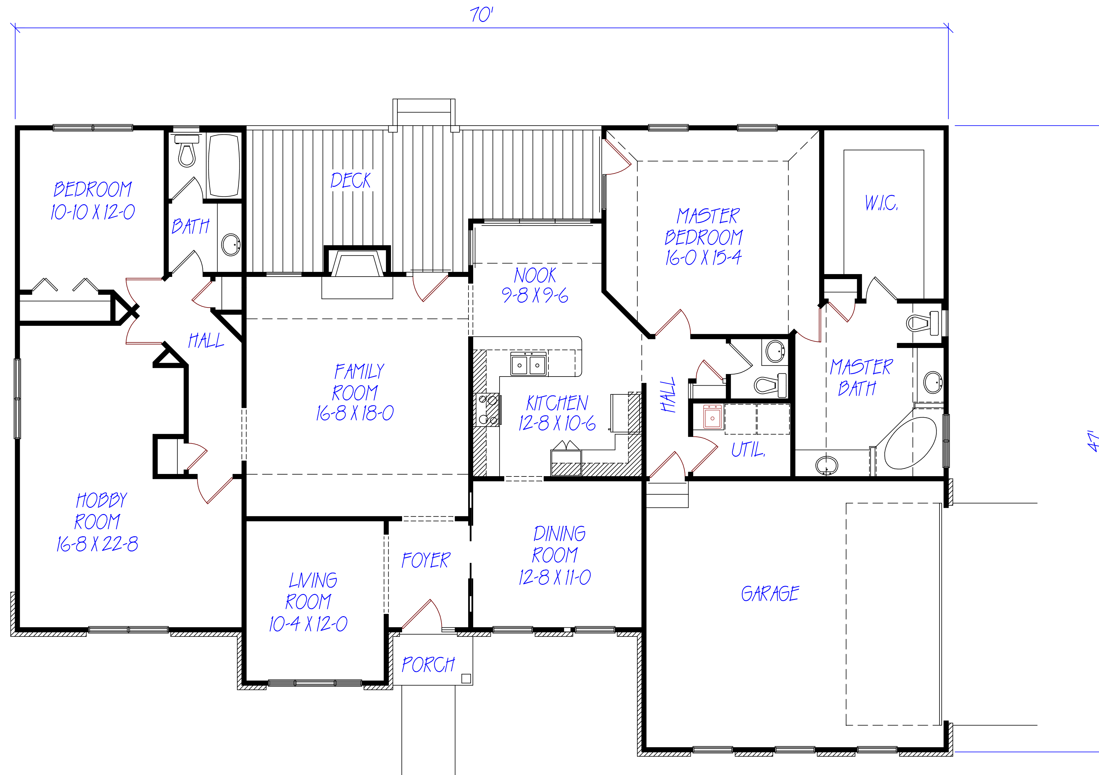
FLOOR PLAN
